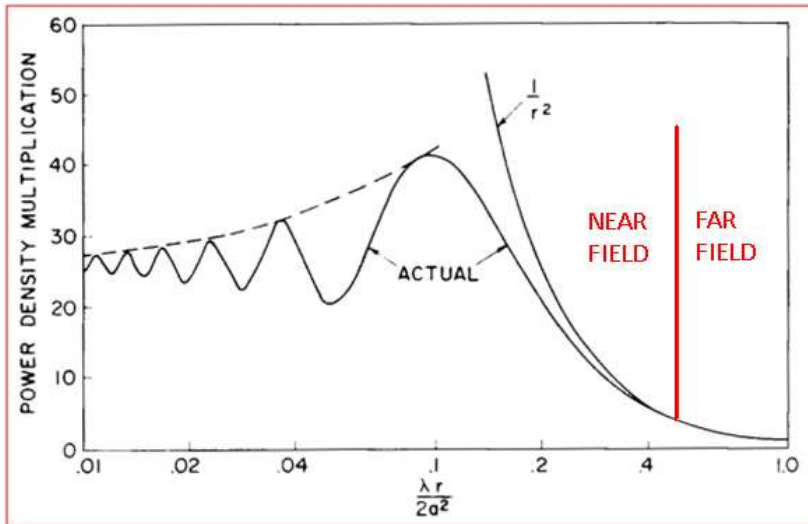
Power density vs distance (r) along the axis of an antenna of diameter a. \lambda is the wavelength of the radiation. The transition distance corresponds to the value 0.5 (at right) on the abscissa of the graph [Polk, 1986].
