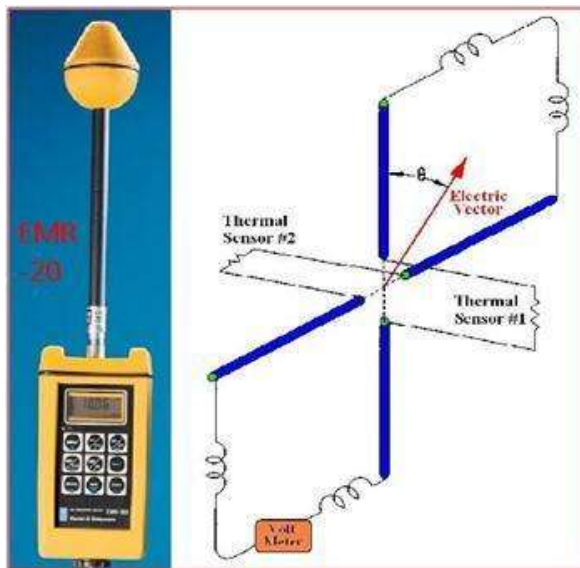
Diagram of 2 (from 3) electric-field measuring dipoles inside an EMR Survey Meter.
