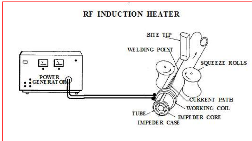
The system uses EMR energy and induction coil to produce seamless pipes or tubes
