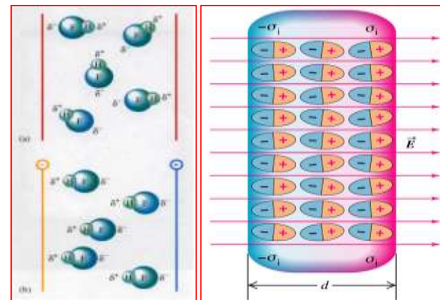
Hydrogen Fluoride molecules are initially randomly oriented (a), and then polarized (b) by an applied Electric Field. Right: a surface charge results.
